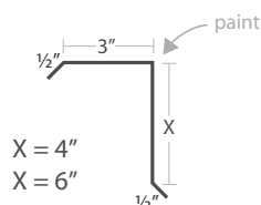
Gable
