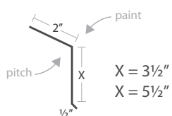
Eave
