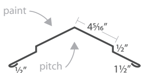
Standard Ridge Cap
