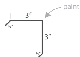
Outside Corner
