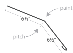
Upper Transition
