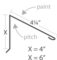
High Eave
