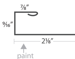
1/2" J-Metal
