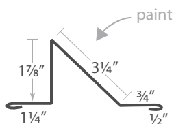
Snow Stop
